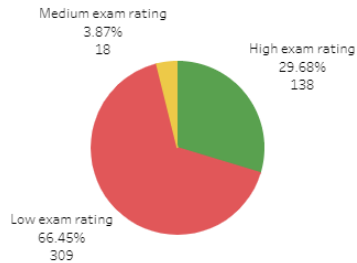
Score distribution
